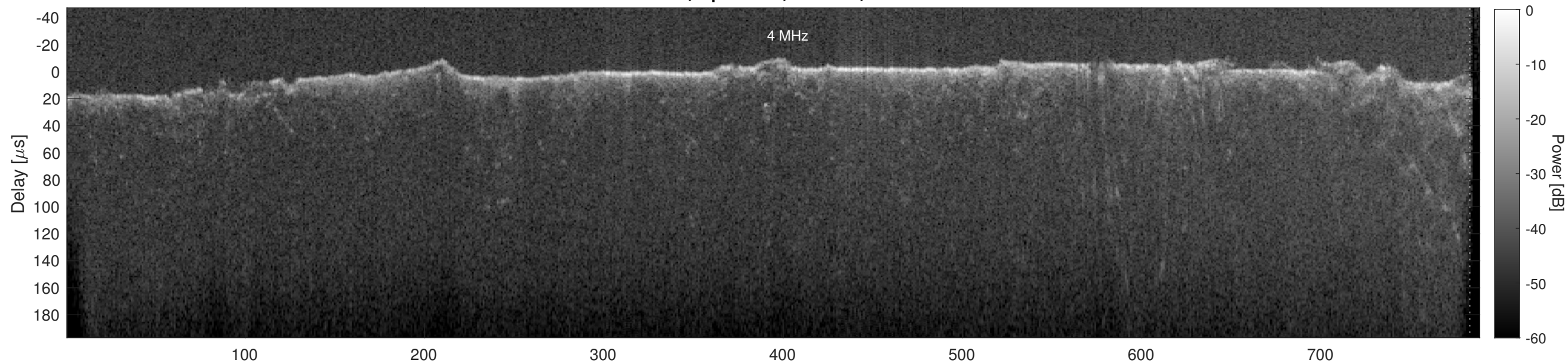
Orbit 19894, Cluttergram
