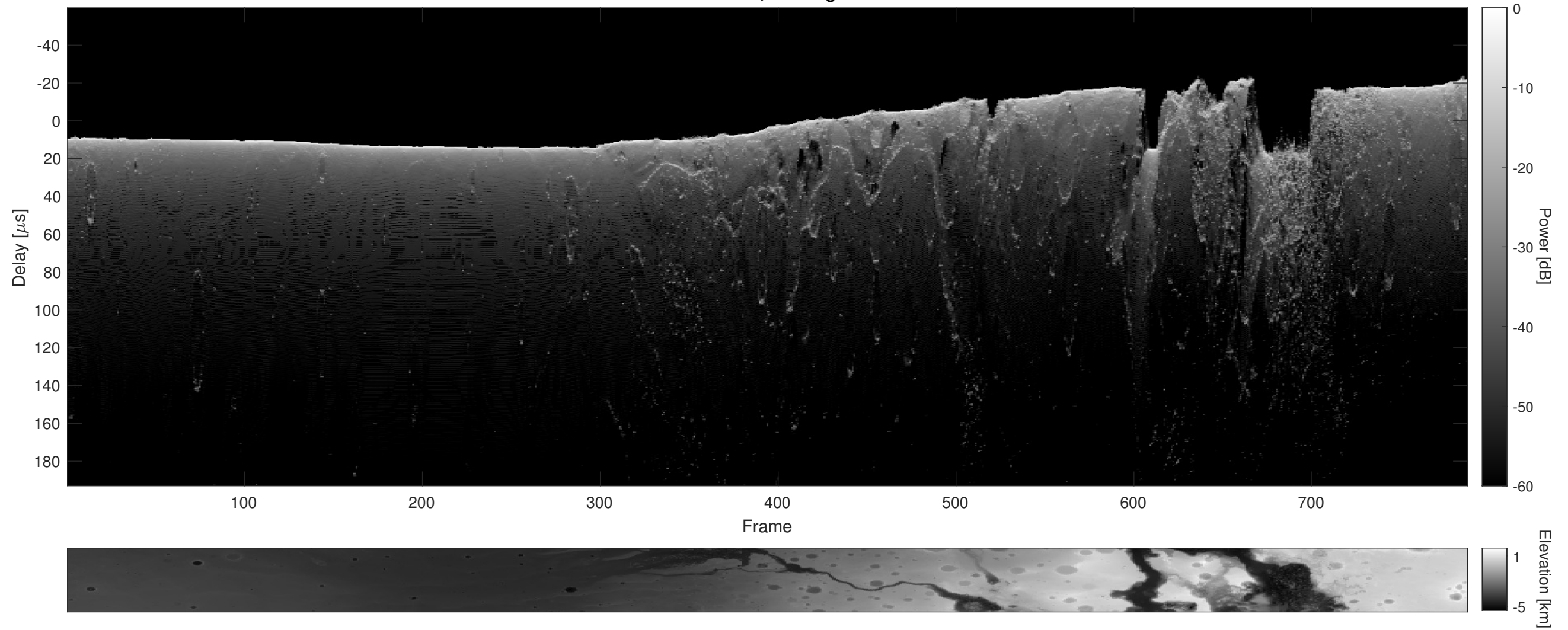
Orbit 19895, Cluttergram
