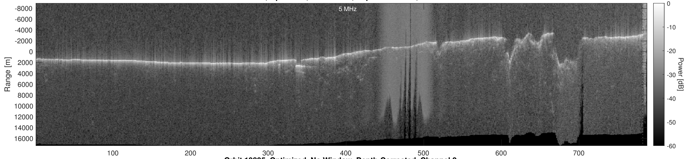
Orbit 19895, Optimized, No Window, Depth-Corrected, Channel 2
