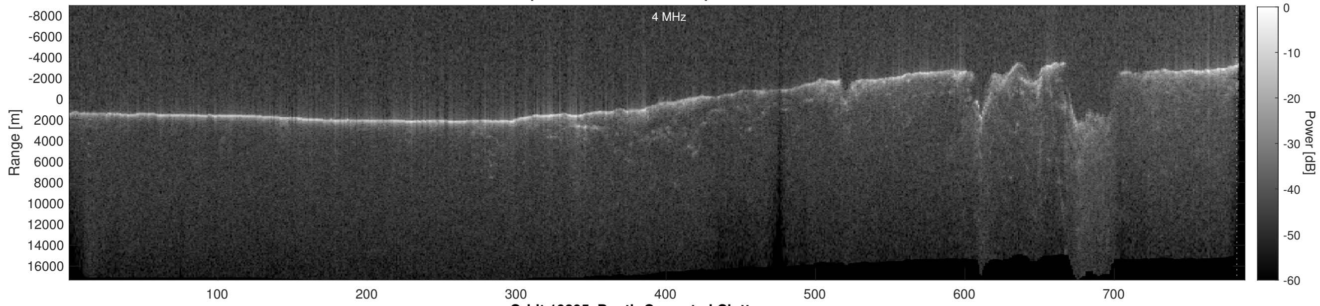
Orbit 19895, Depth-Corrected Cluttergram
