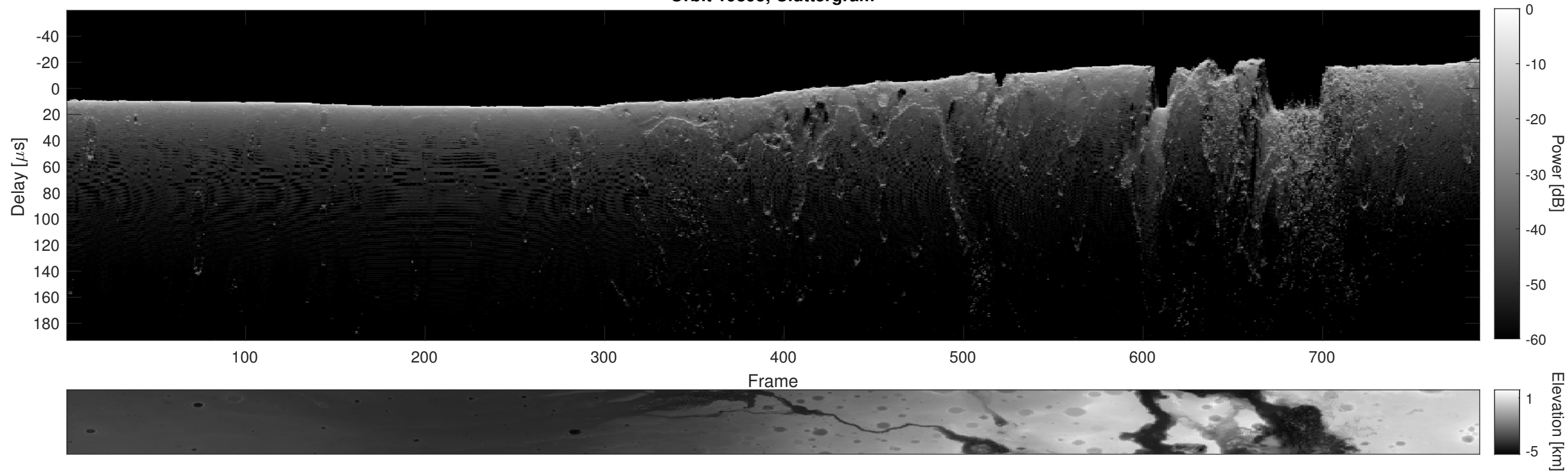
Orbit 19895, Cluttergram
