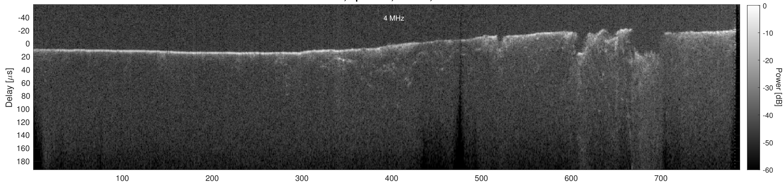
Orbit 19895, Cluttergram
