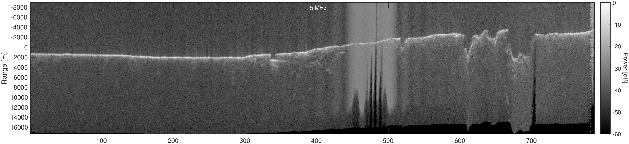
Orbit 19895, Optimized, Window, Depth-Corrected, Channel 2
