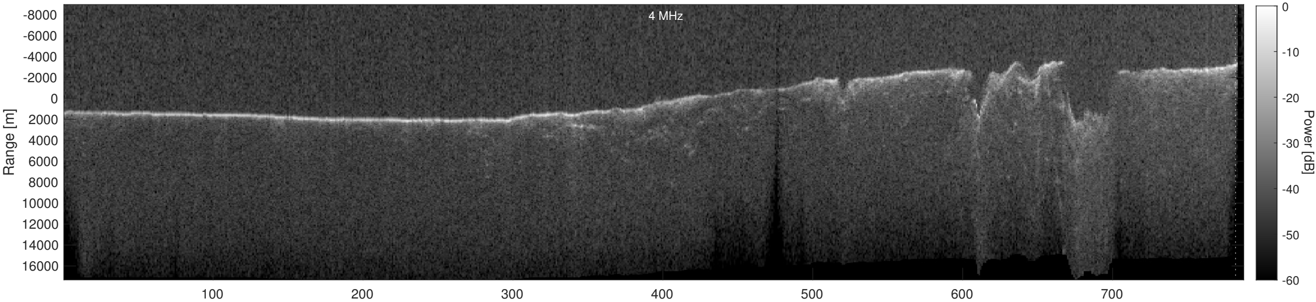
Orbit 19895, Depth-Corrected Cluttergram
