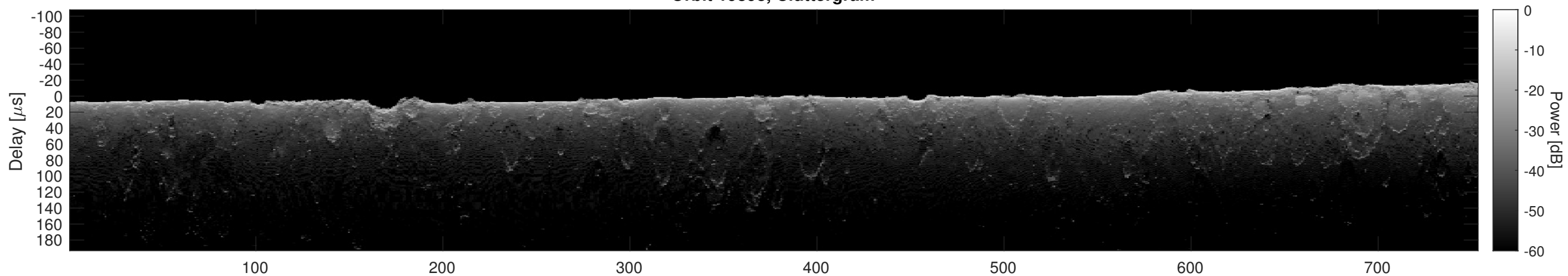
Orbit 19898, Cluttergram
