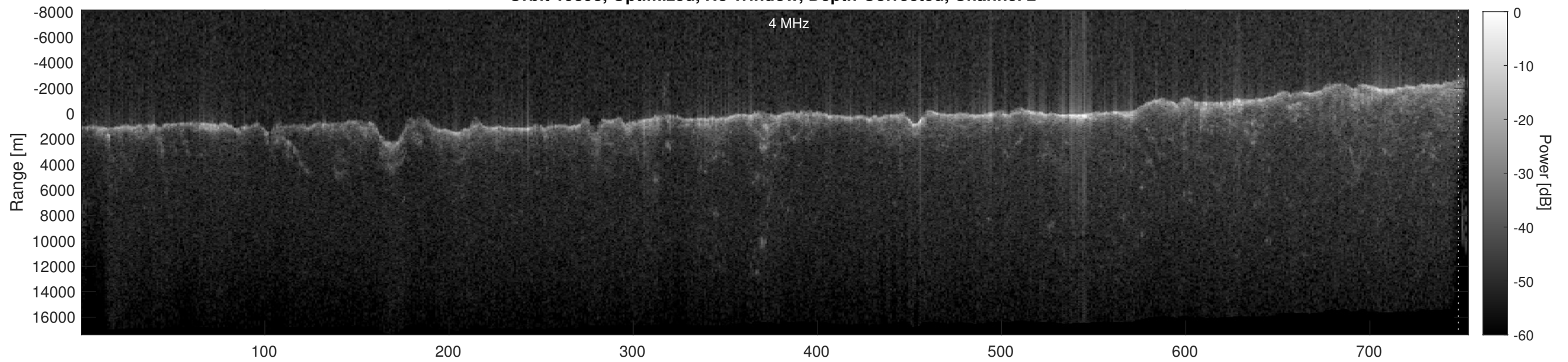
Orbit 19898, Depth-Corrected Cluttergram
