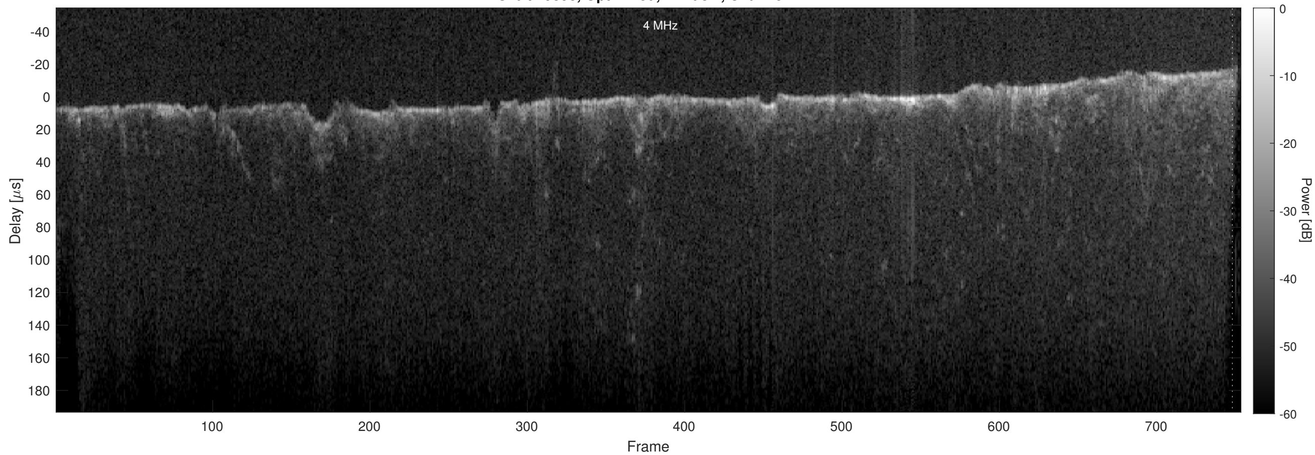
Orbit 19898, Optimized, Window, Channel 2
