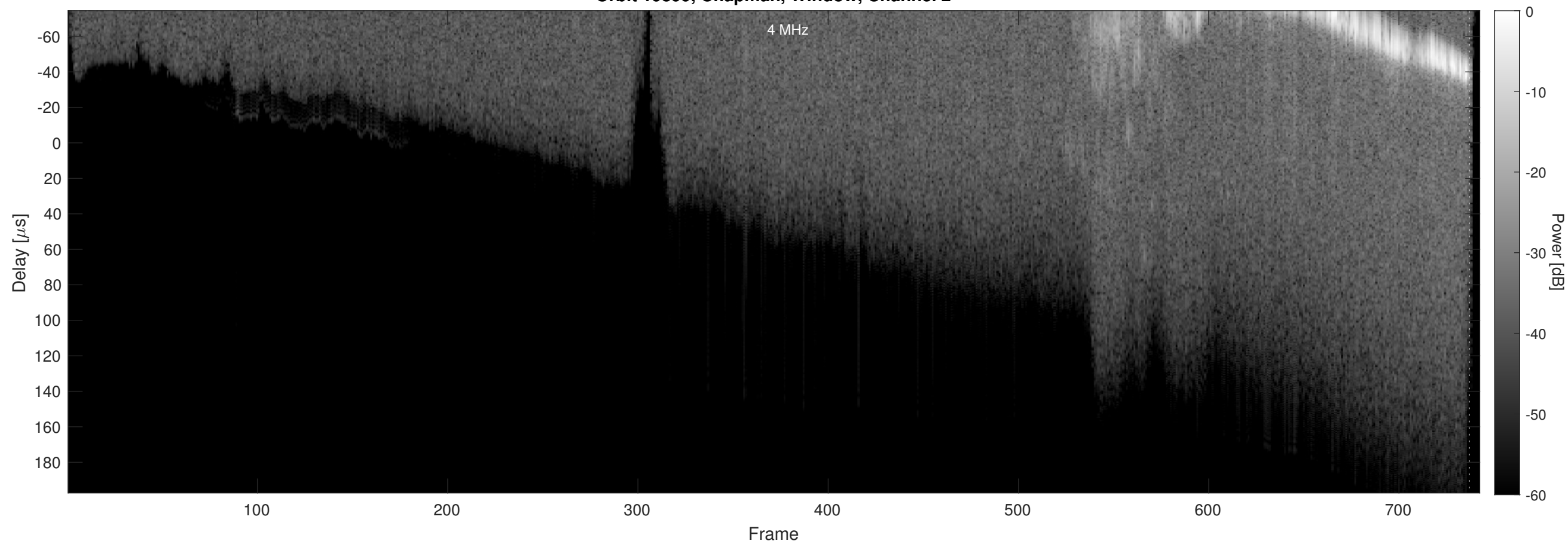
Orbit 19899, Chapman, Window, Channel 2
