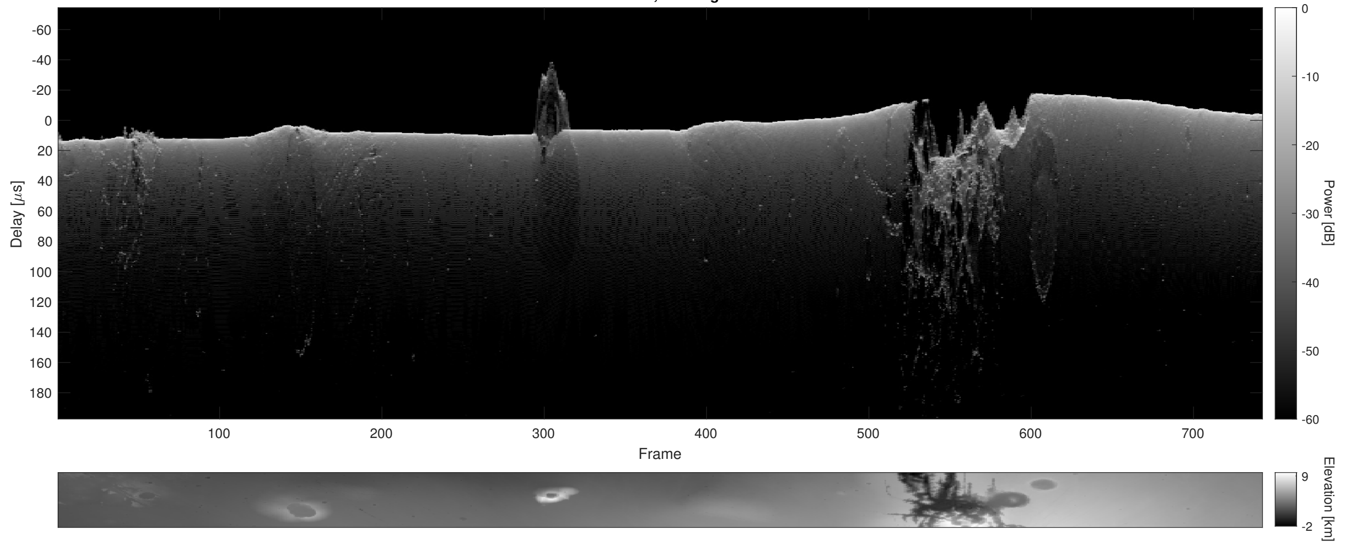
Orbit 19899, Cluttergram
