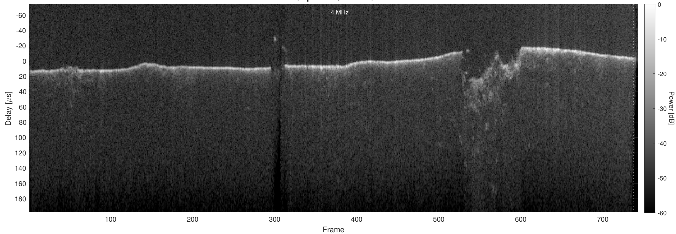
Orbit 19899, Optimized, Window, Channel 2
