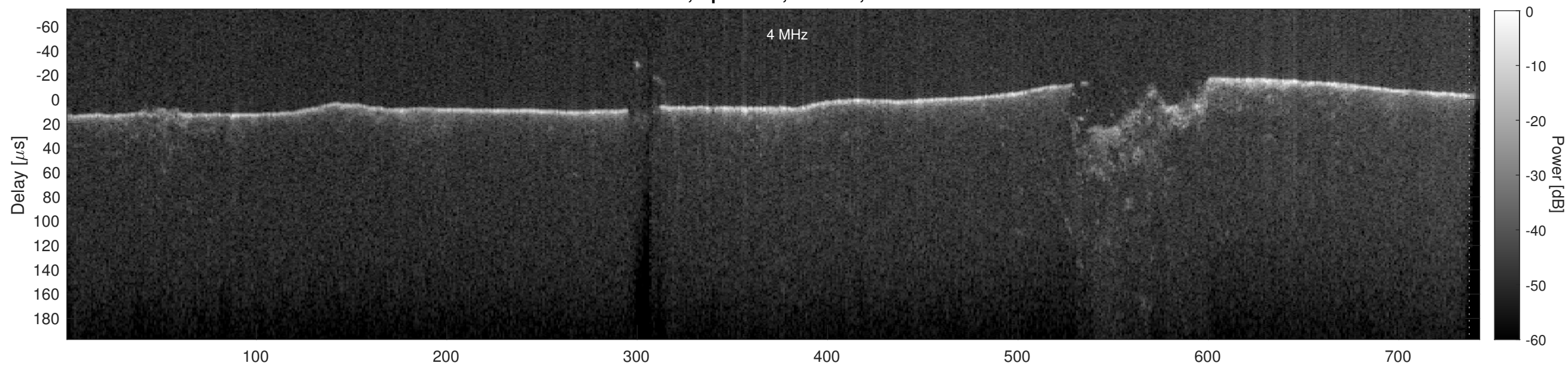
Orbit 19899, Cluttergram
