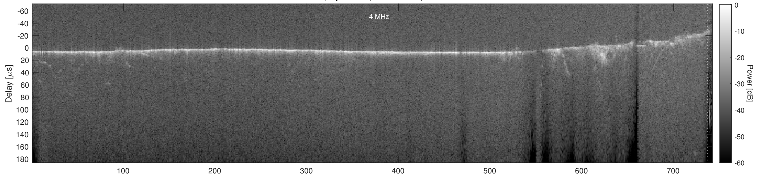
Orbit 19900, Cluttergram
