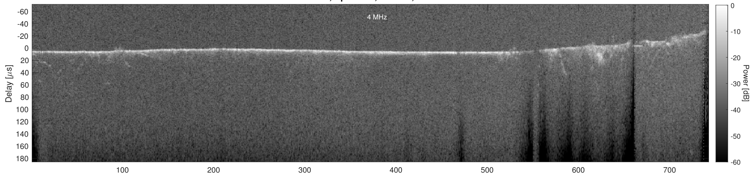
Orbit 19900, Cluttergram
