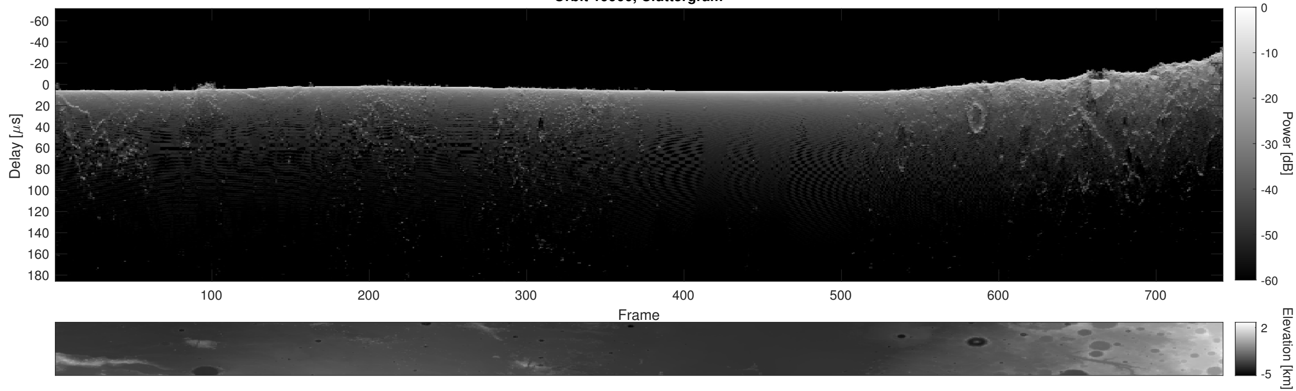
Orbit 19900, Cluttergram
