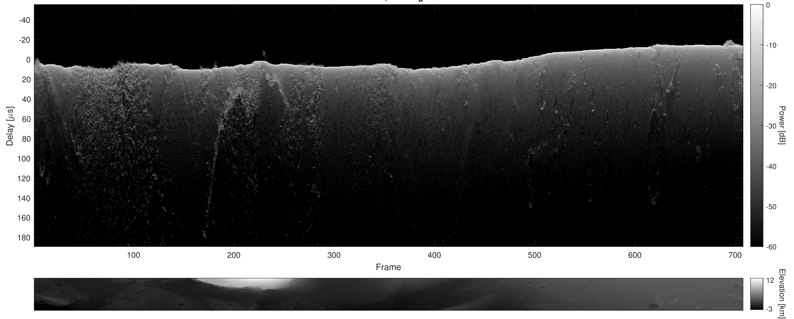
Orbit 19903, Cluttergram
