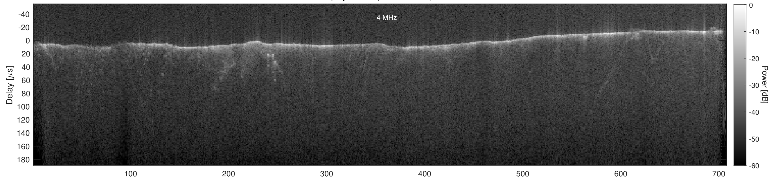
Orbit 19903, Cluttergram
