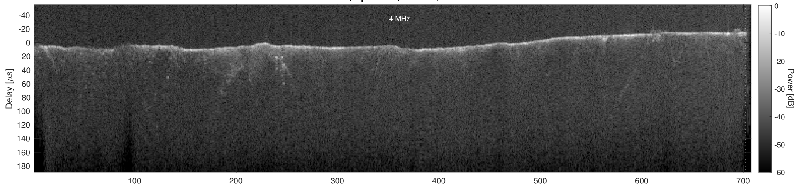
Orbit 19903, Cluttergram
