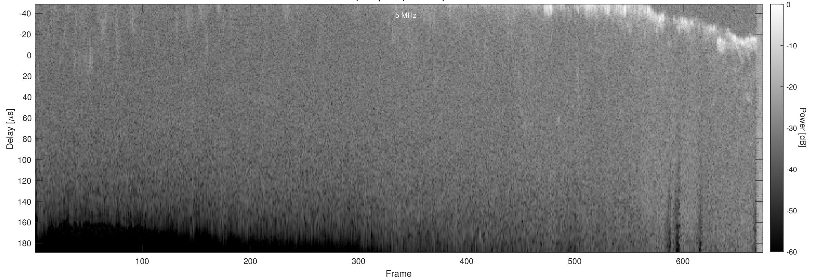
Orbit 19908, Chapman, Window, Channel 2
