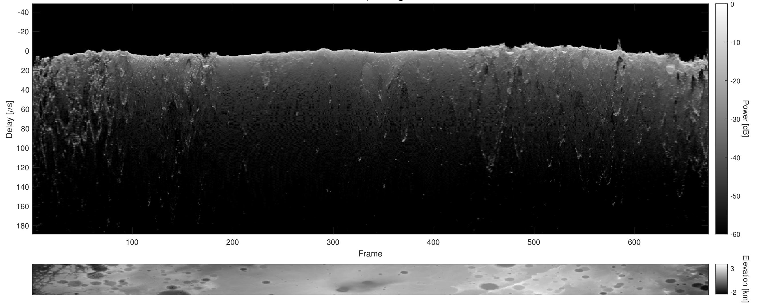
Orbit 19908, Cluttergram
