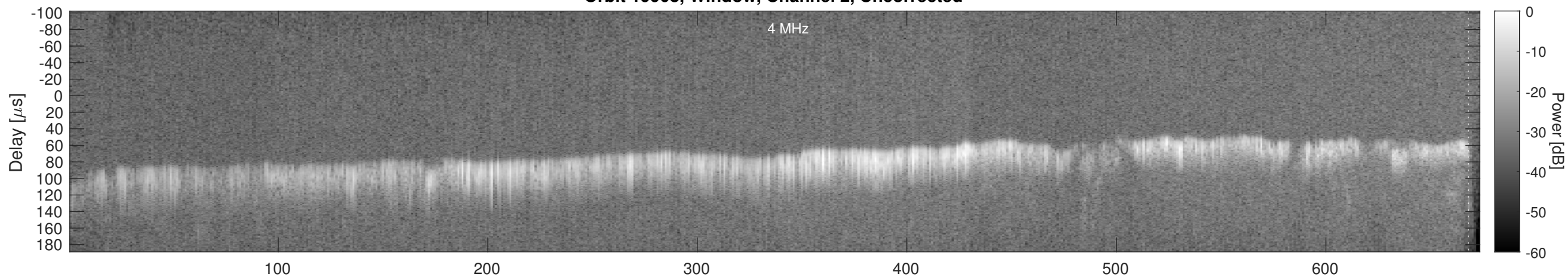
Orbit 19908, Window, Channel 2, Chapman
