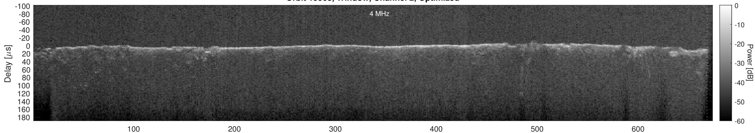
Orbit 19908, Cluttergram
