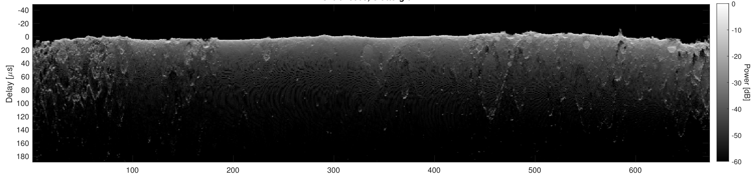
Orbit 19908, Cluttergram
