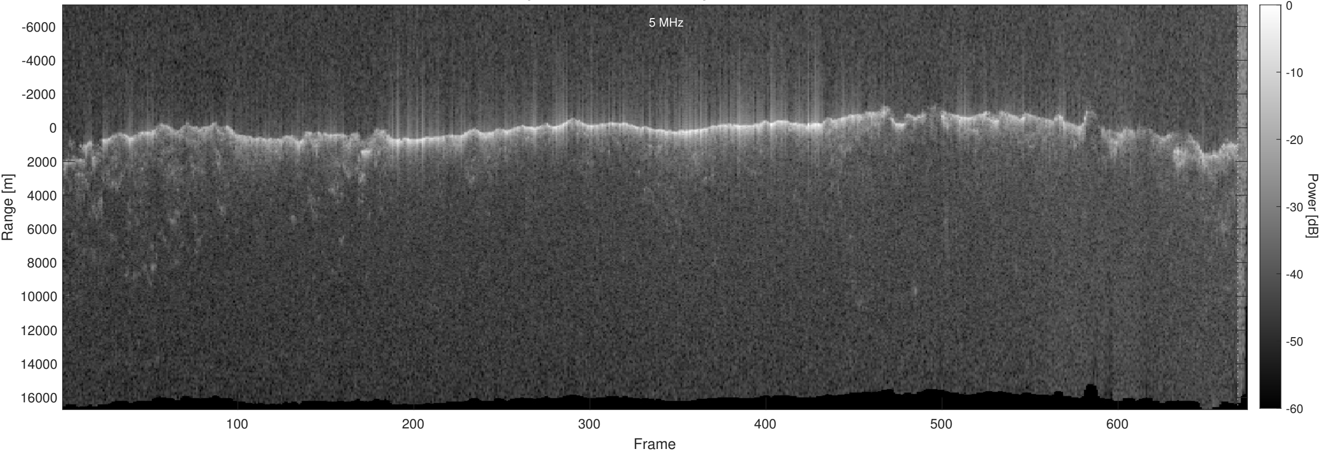
Orbit 19908, Optimized, No Window, Depth-Corrected, Channel 2
