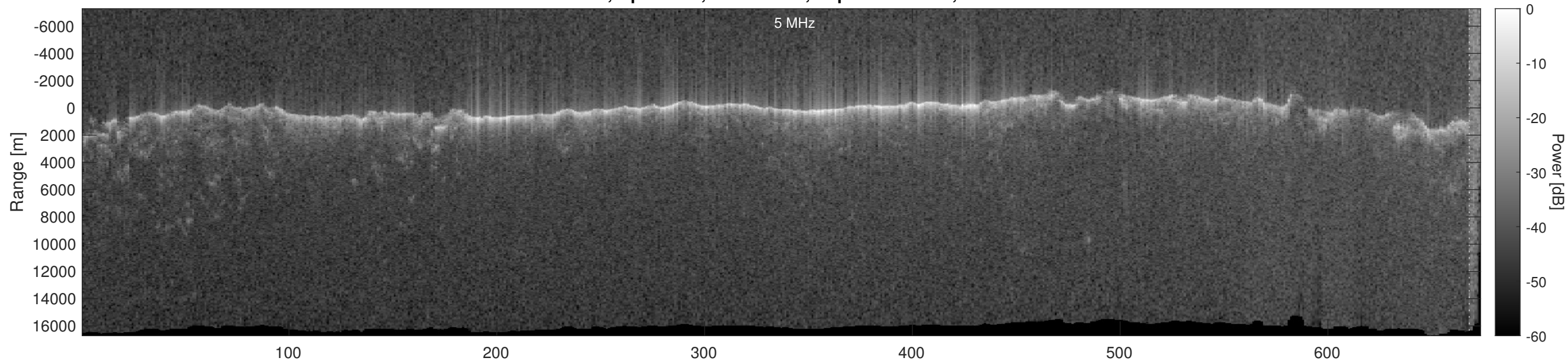
Orbit 19908, Optimized, No Window, Depth-Corrected, Channel 2
