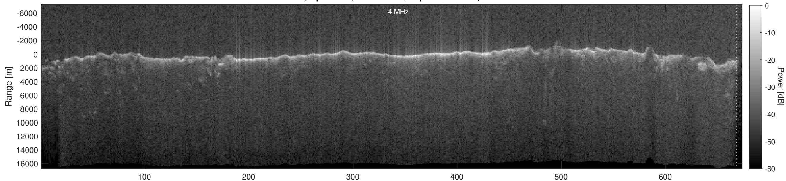
Orbit 19908, Depth-Corrected Cluttergram
