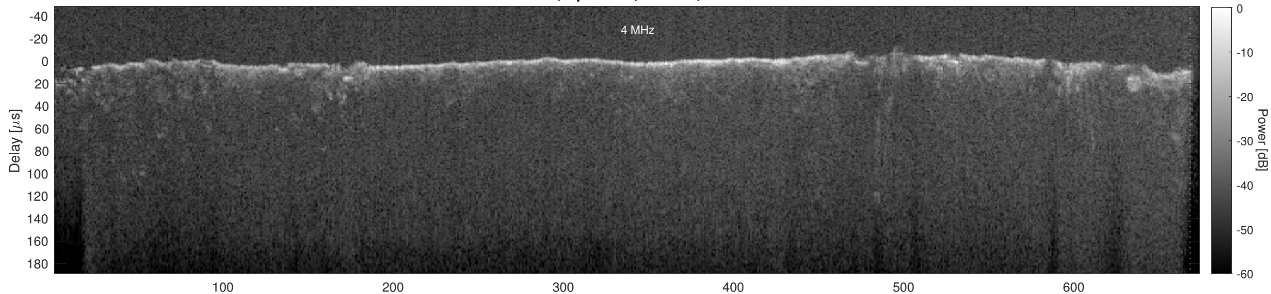
Orbit 19908, Cluttergram
