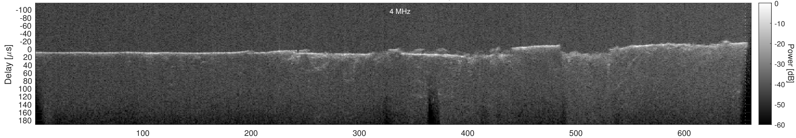
Orbit 19909, Cluttergram
