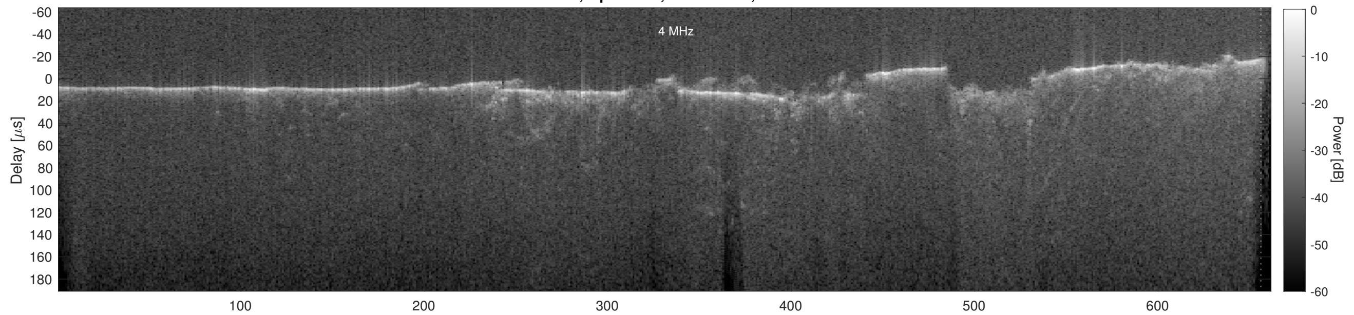
Orbit 19909, Cluttergram
