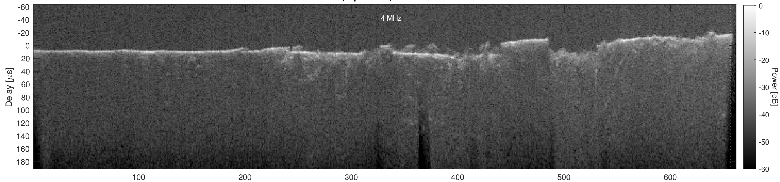
Orbit 19909, Cluttergram
