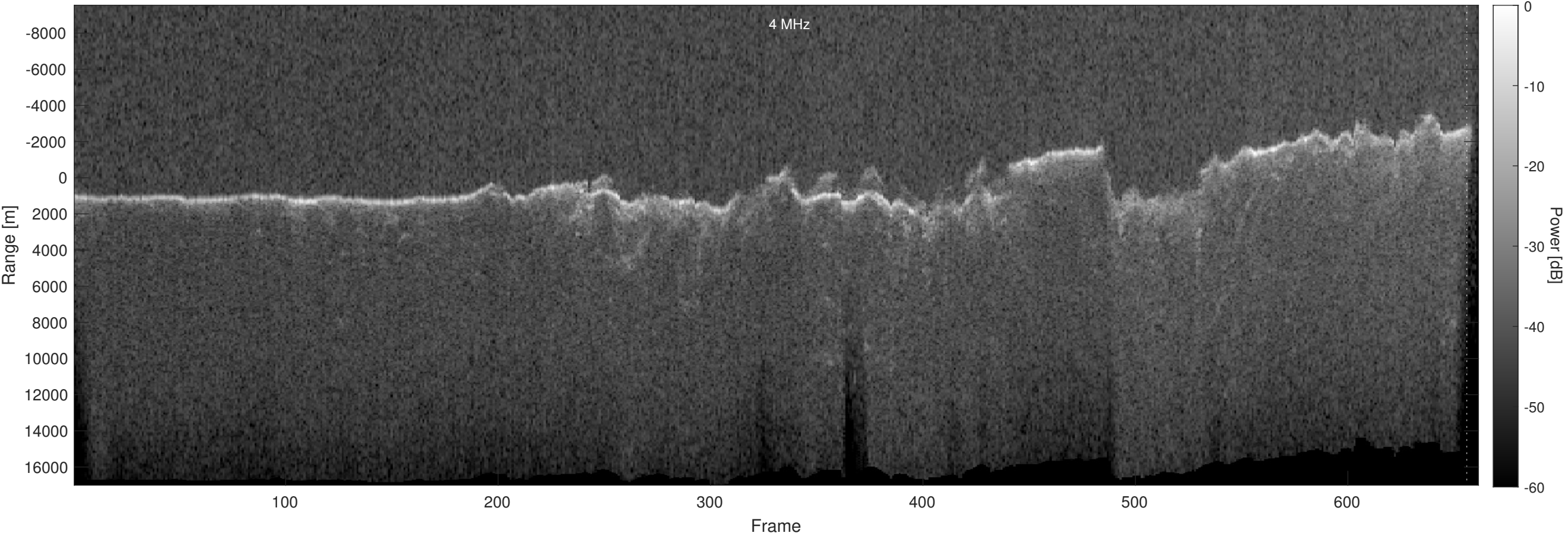
Orbit 19909, Optimized, Window, Depth-Corrected, Channel 2
