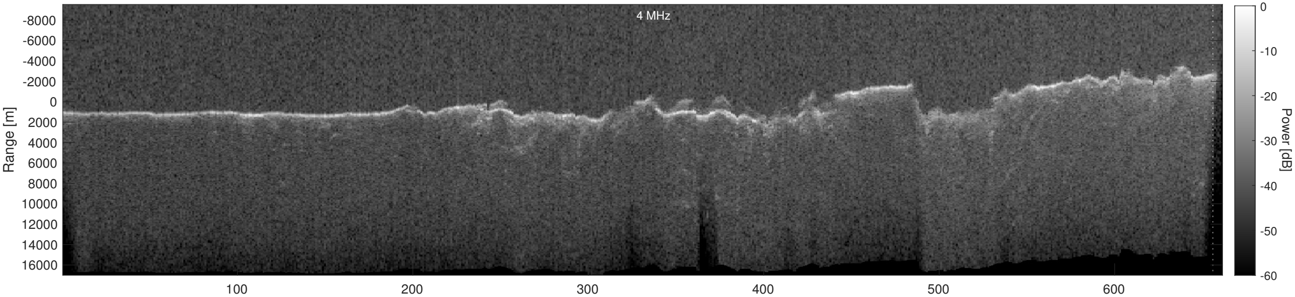
Orbit 19909, Depth-Corrected Cluttergram
