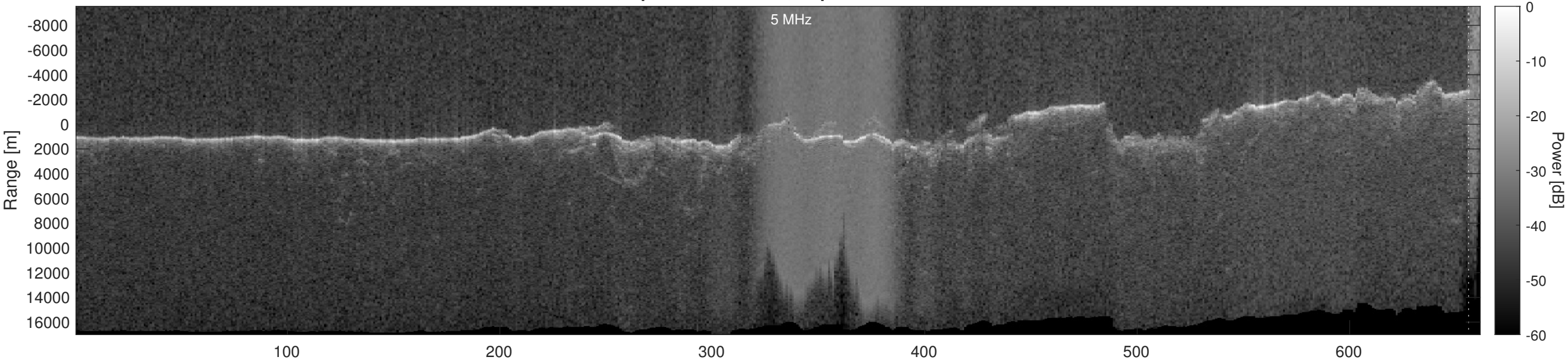
Orbit 19909, Optimized, Window, Depth-Corrected, Channel 2
