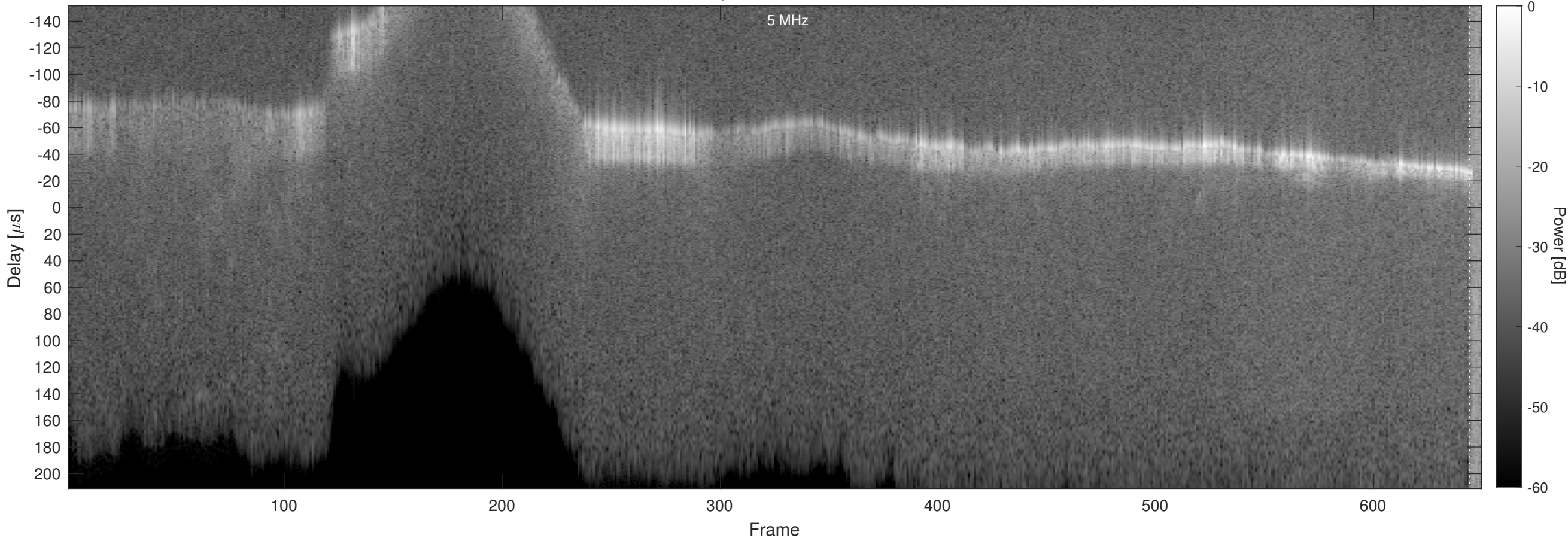
Orbit 19910, Chapman, No Window, Channel 2
