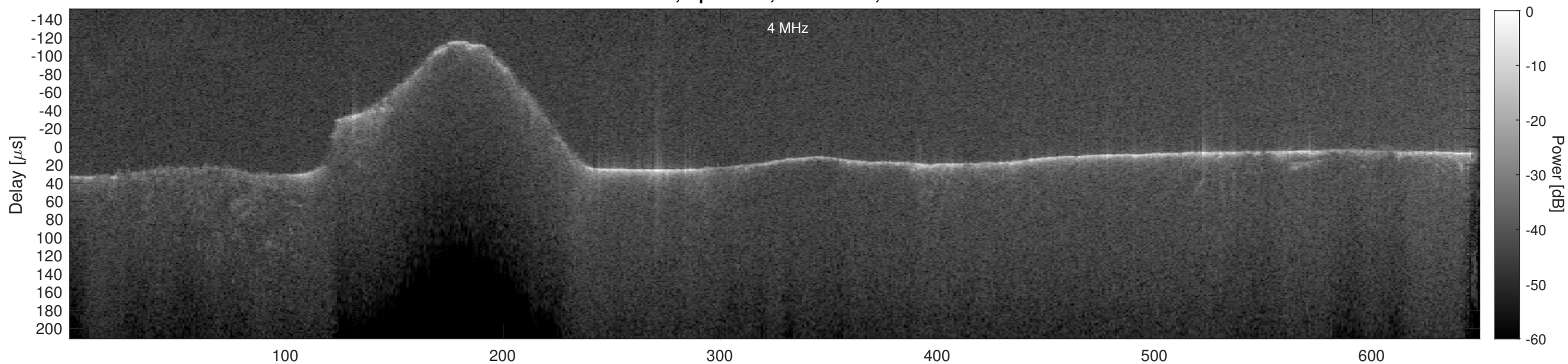
Orbit 19910, Cluttergram
