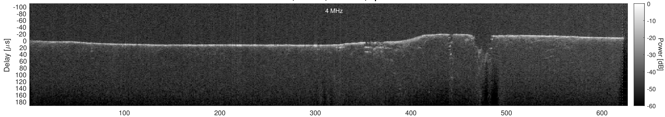
Orbit 19913, Cluttergram
