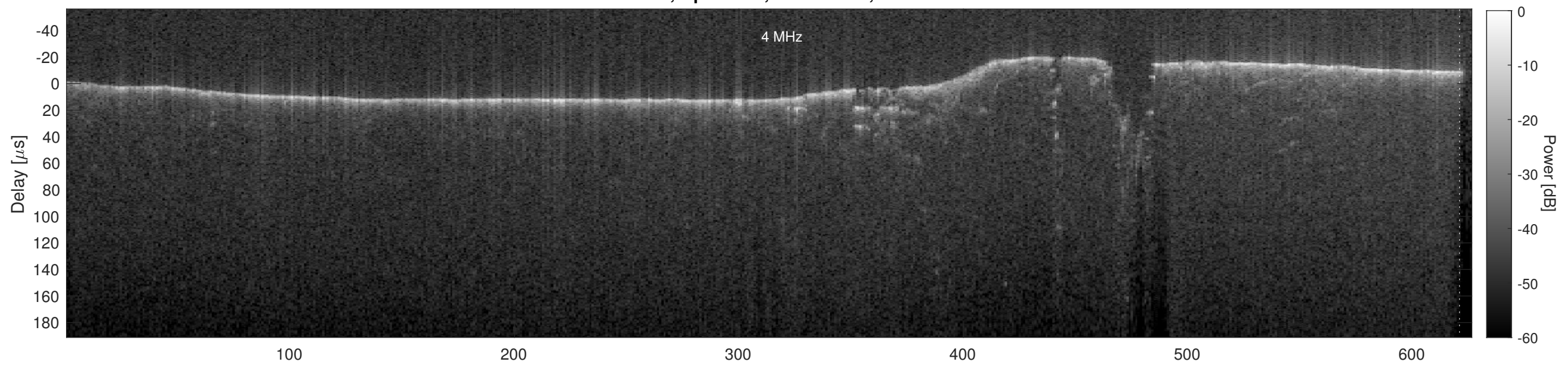
Orbit 19913, Cluttergram
