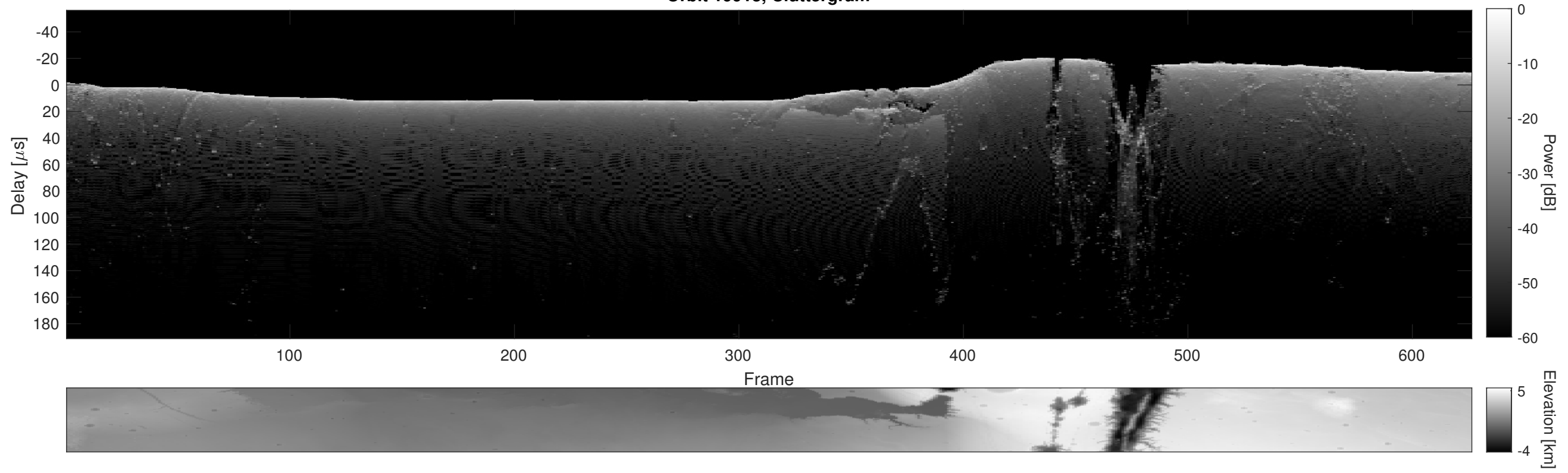
Orbit 19913, Cluttergram
