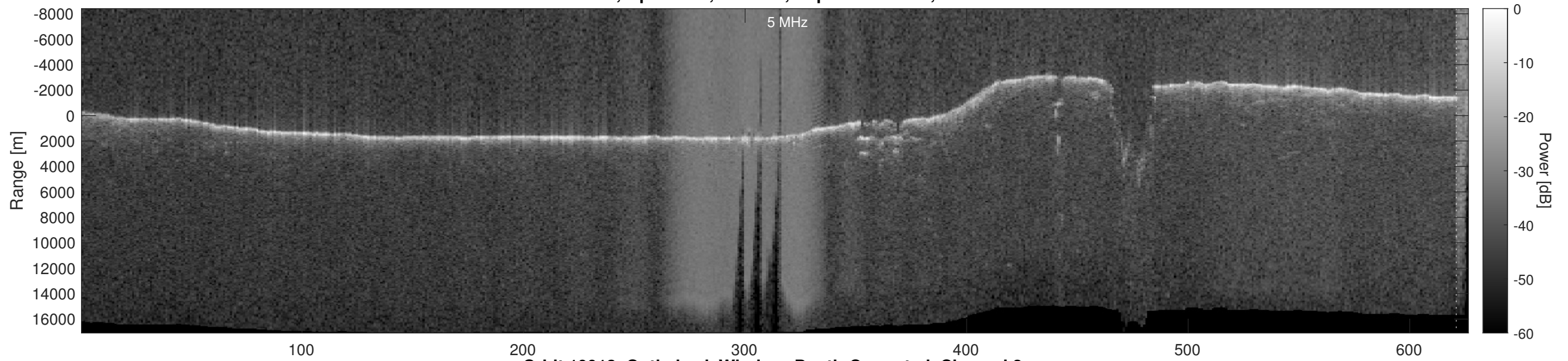
Orbit 19913, Optimized, Window, Depth-Corrected, Channel 2
