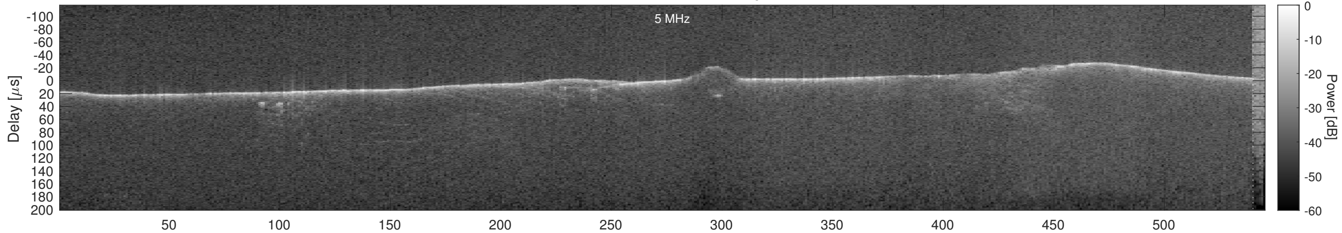
Orbit 19924, Cluttergram
