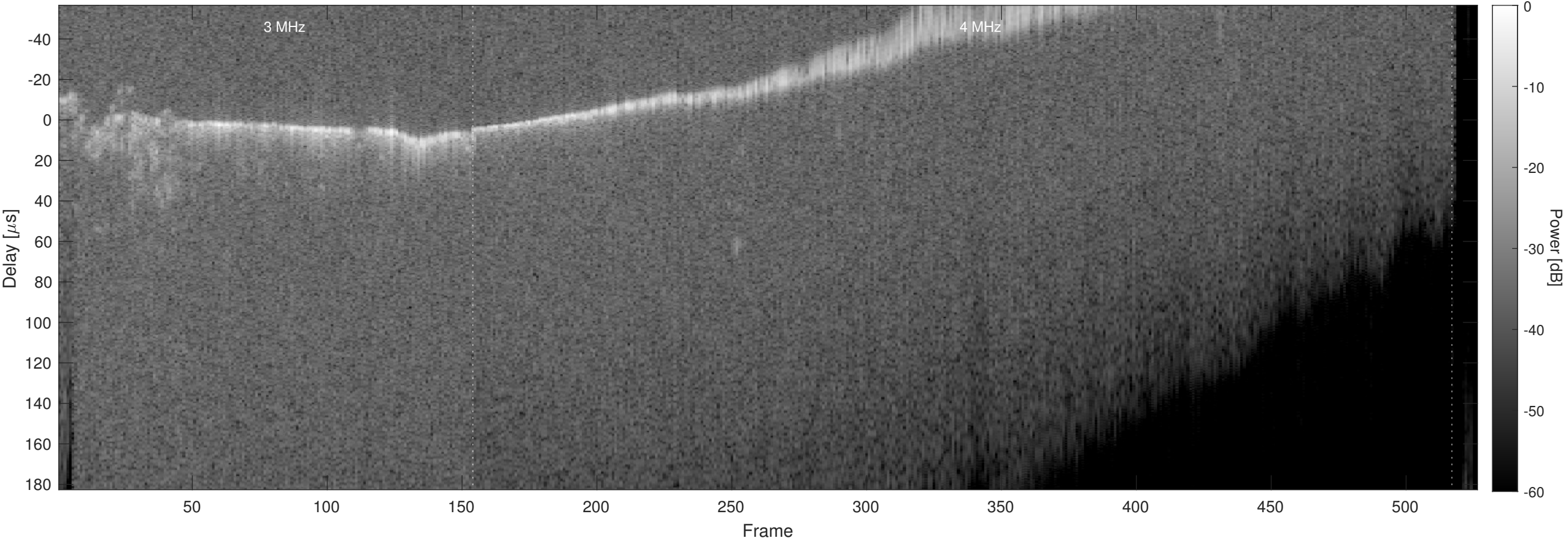
Orbit 20238, Chapman, No Window, Channel 2
