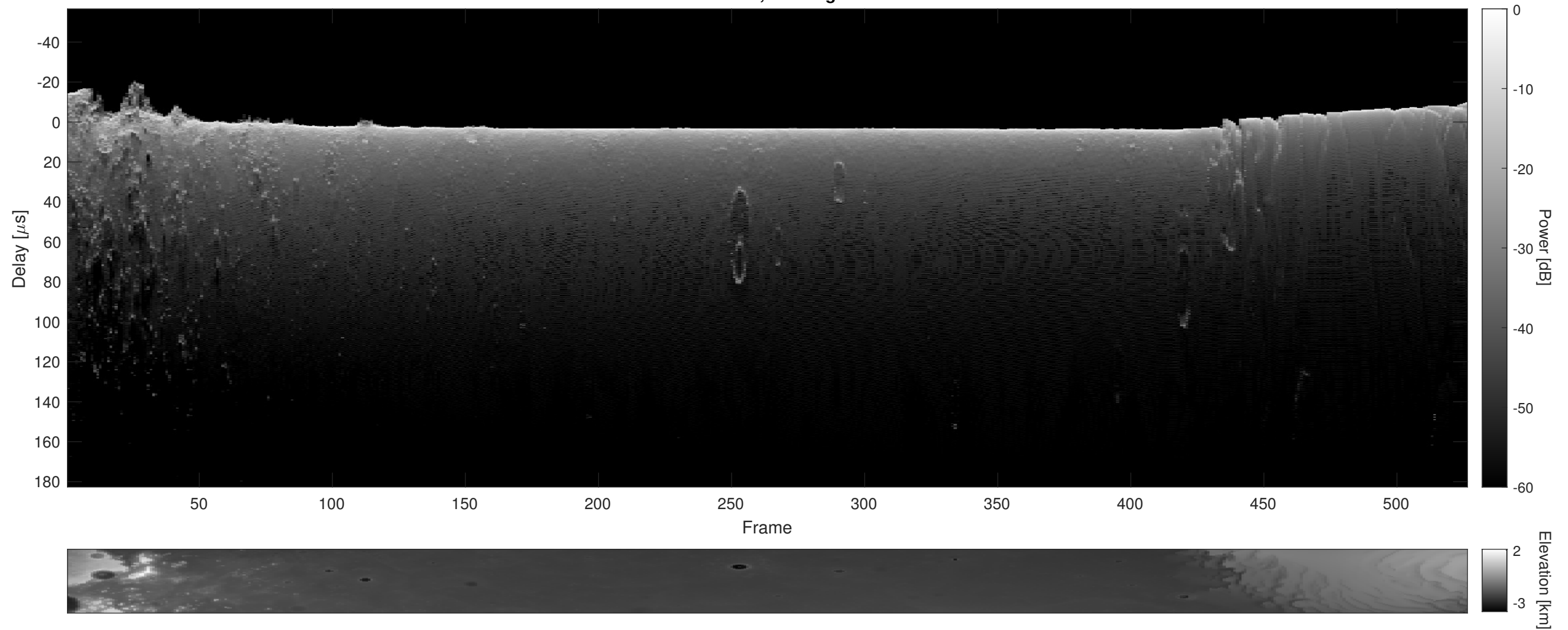
Orbit 20238, Cluttergram
