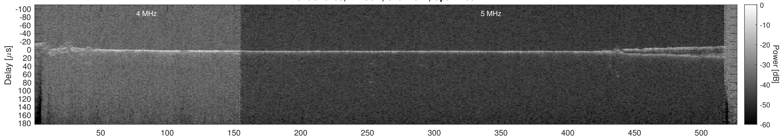
Orbit 20238, Cluttergram
