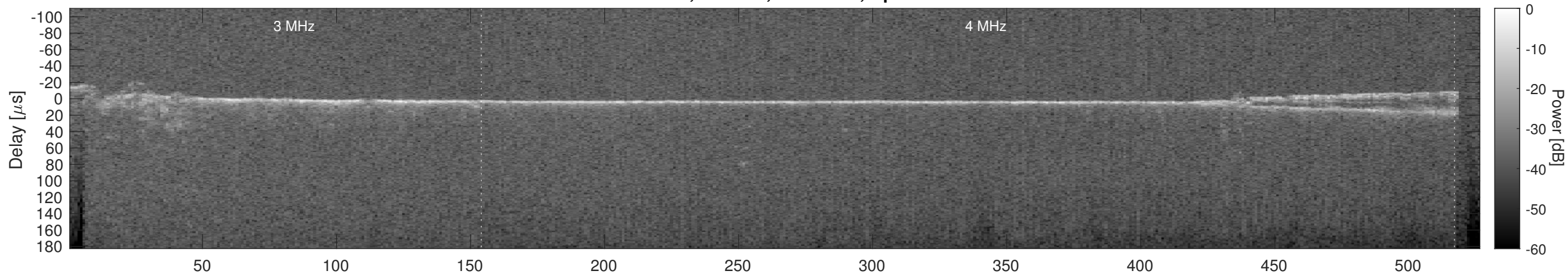
Orbit 20238, Cluttergram
