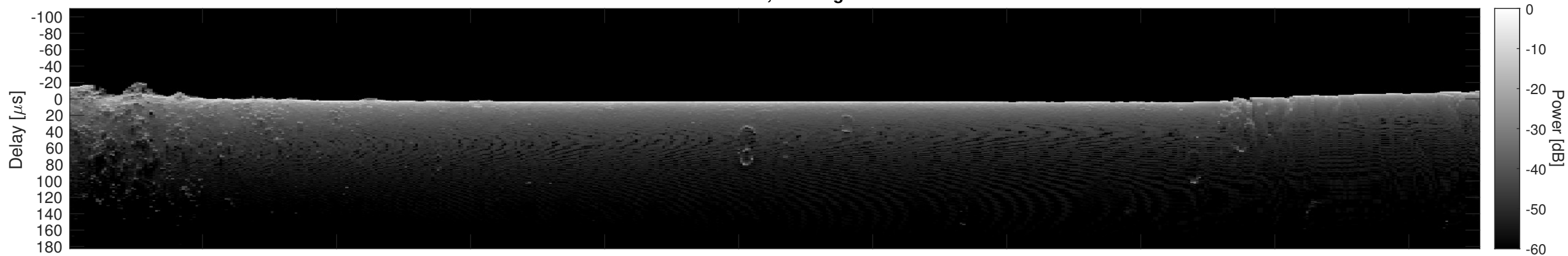
Orbit 20238, Cluttergram
