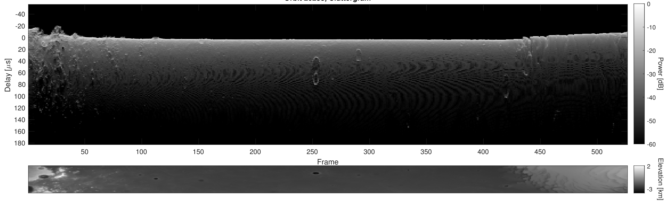
Orbit 20238, Cluttergram
