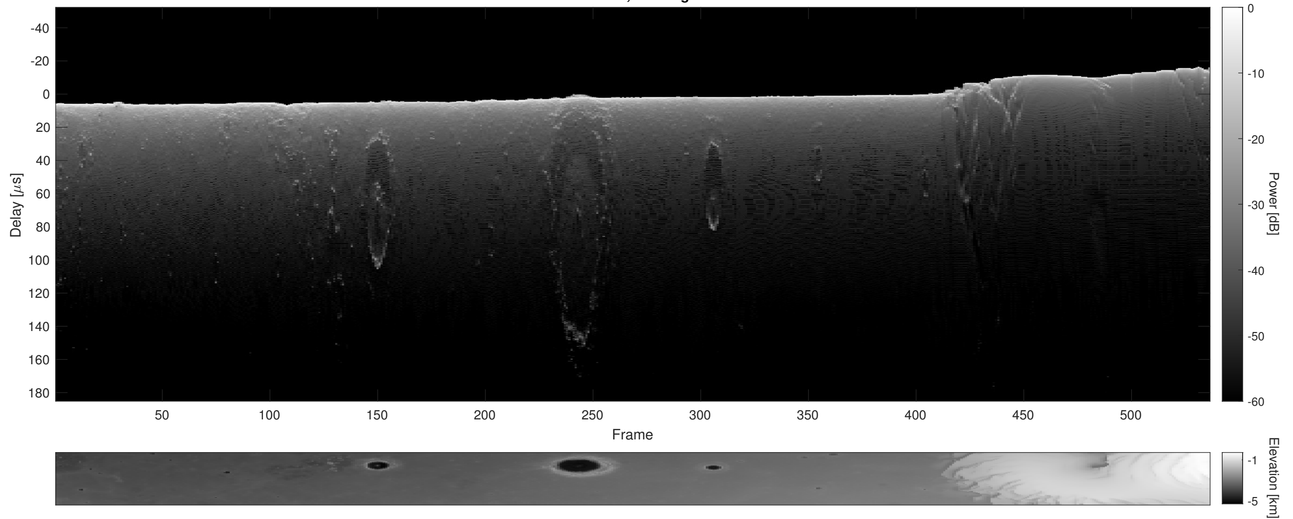
Orbit 20242, Cluttergram
