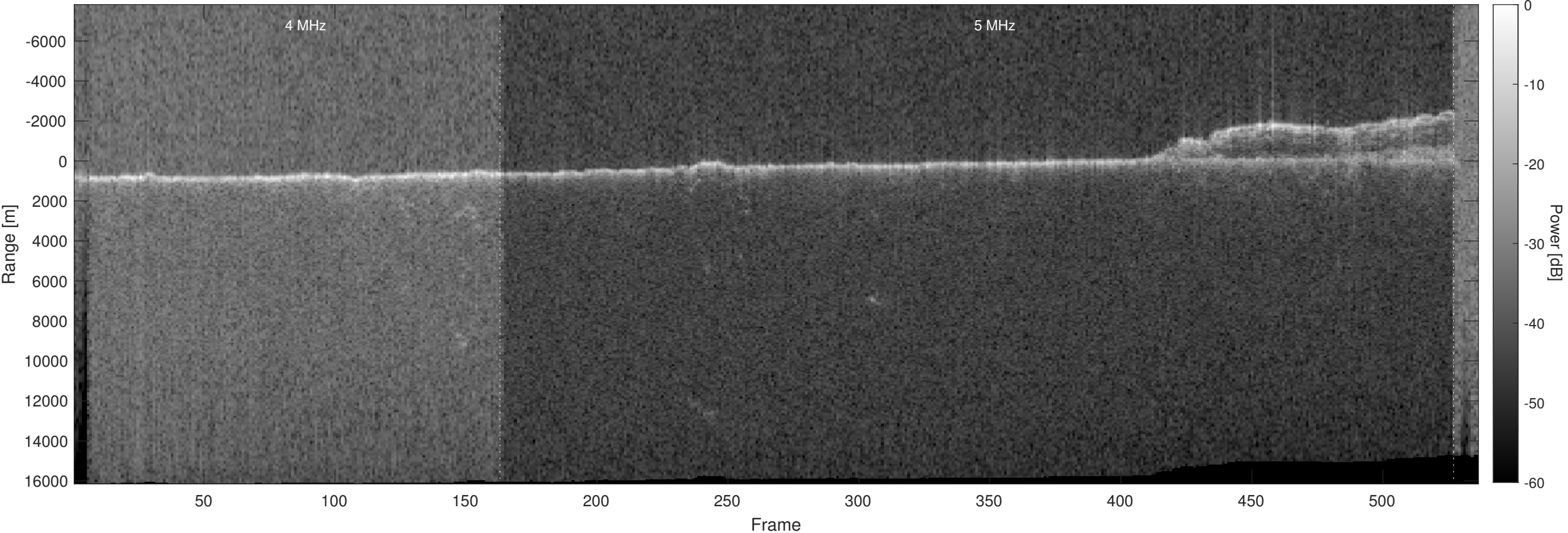
Orbit 20242, Optimized, Window, Depth-Corrected, Channel 2
