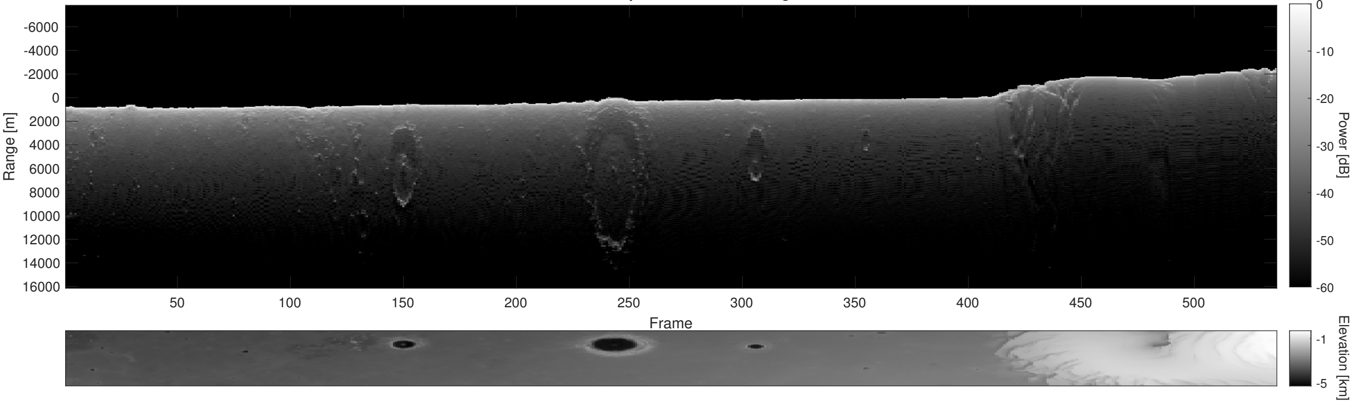
Orbit 20242, Depth-Corrected Cluttergram
