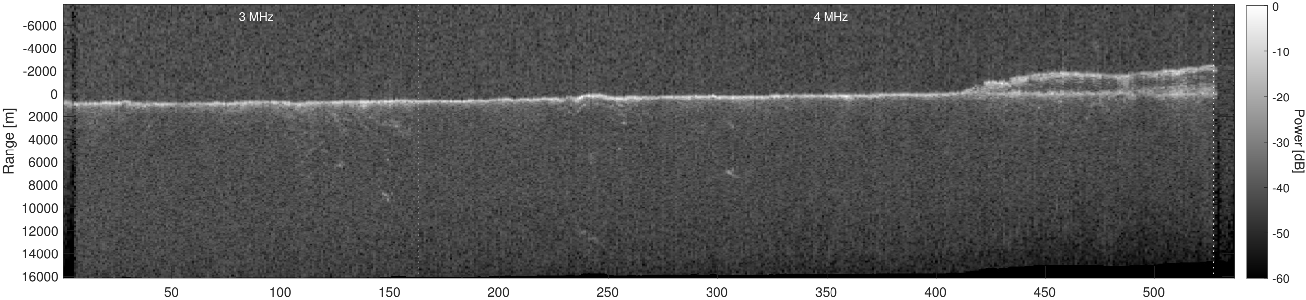
Orbit 20242, Depth-Corrected Cluttergram
