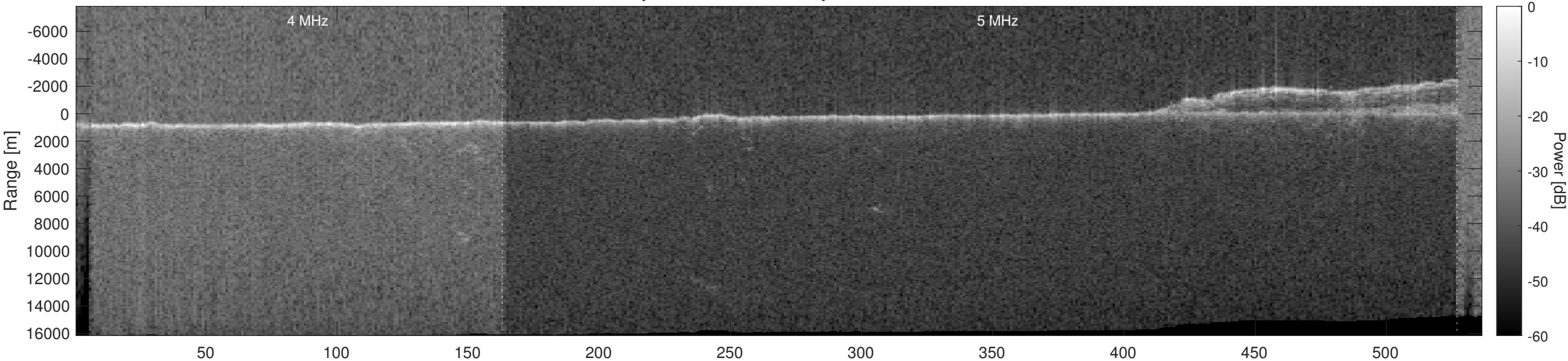
Orbit 20242, Optimized, Window, Depth-Corrected, Channel 2
