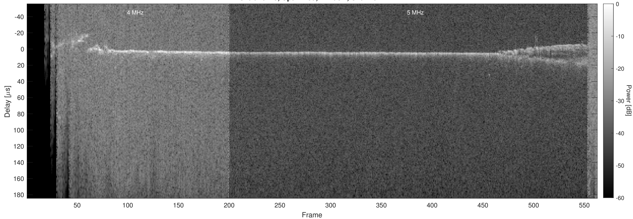
Orbit 20245, Optimized, Window, Channel 2
