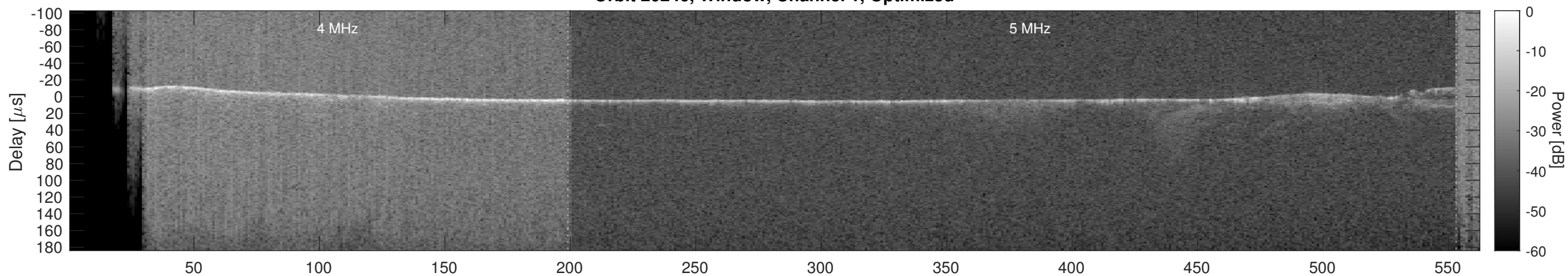
Orbit 20246, Cluttergram
