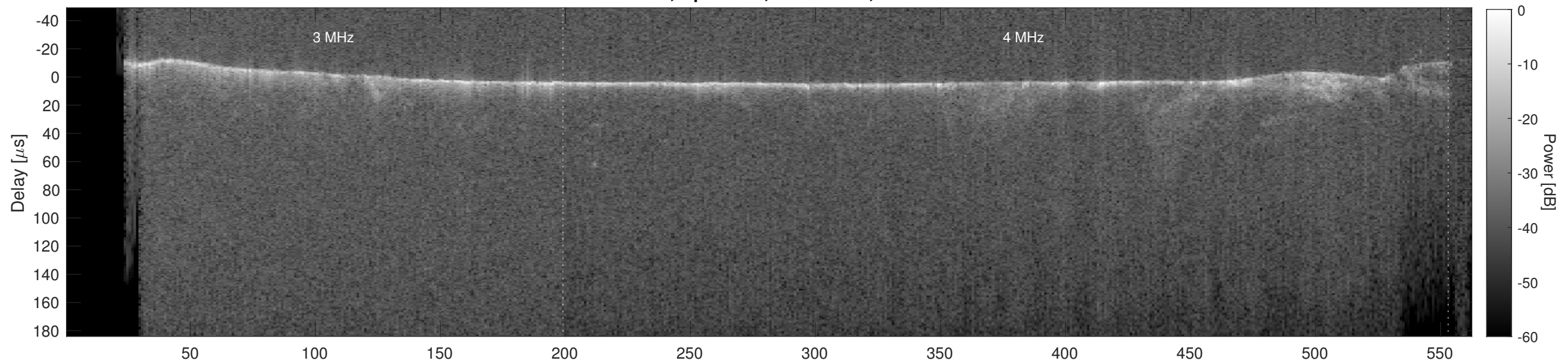
Orbit 20246, Cluttergram
