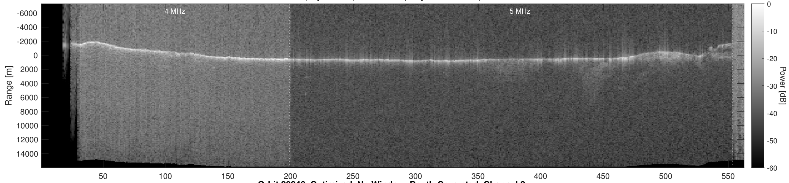
Orbit 20246, Optimized, No Window, Depth-Corrected, Channel 2
