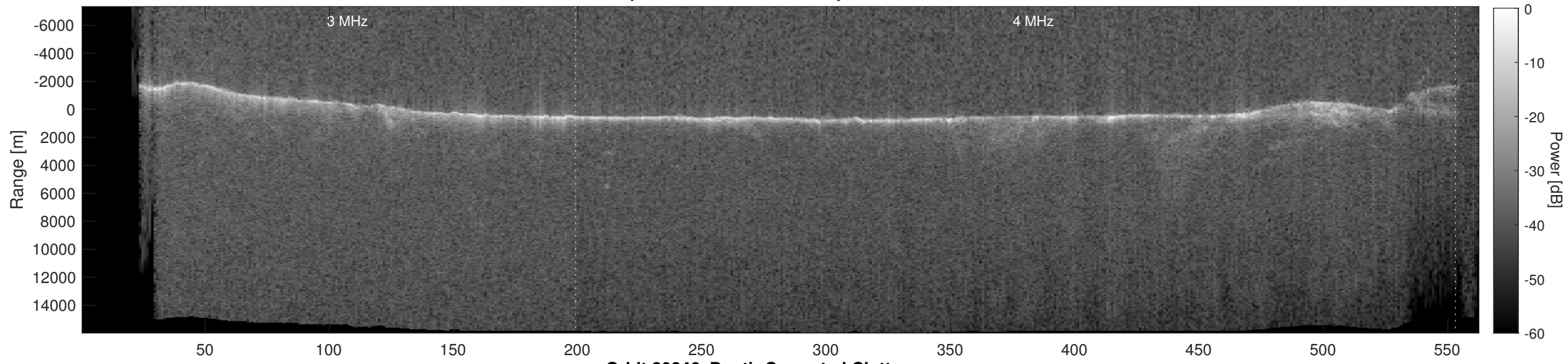
Orbit 20246, Depth-Corrected Cluttergram
