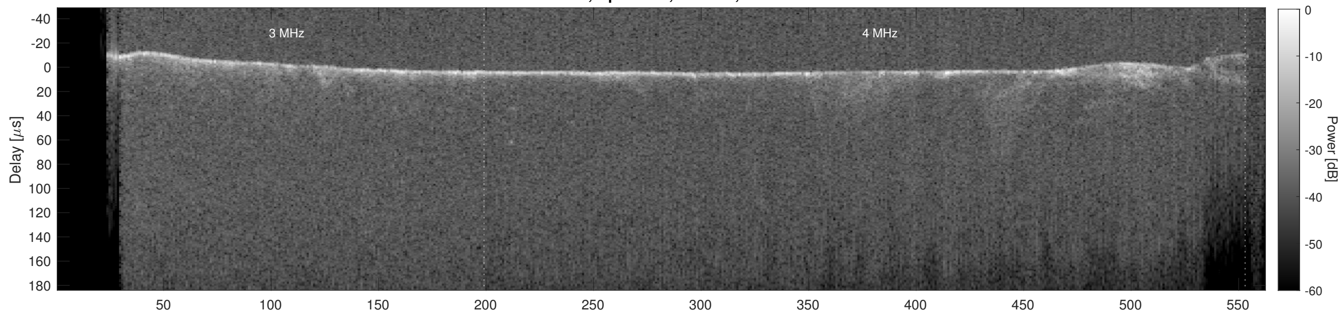
Orbit 20246, Cluttergram
