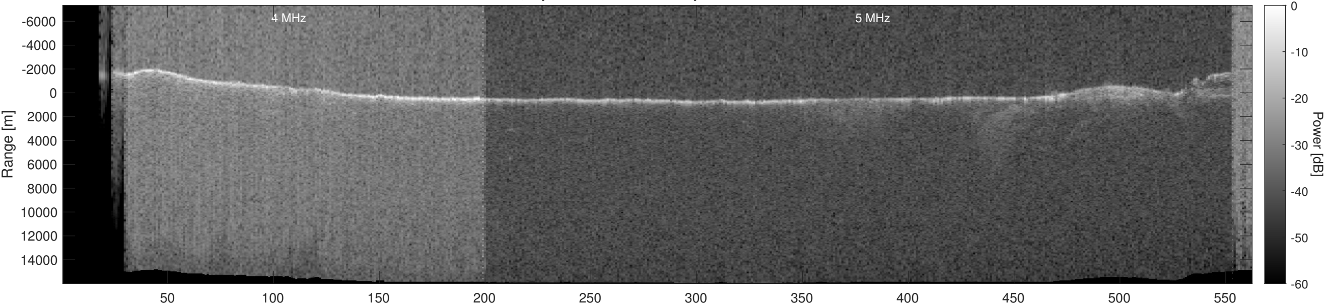
Orbit 20246, Optimized, Window, Depth-Corrected, Channel 2
