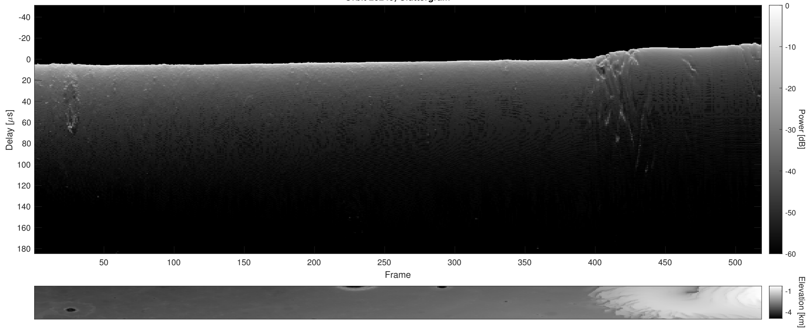
Orbit 20249, Cluttergram
